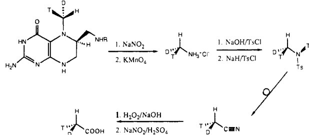
Scheme III. Sequence of Reactions Used To Convert Methyl tetrahydrofolate to Acetate
